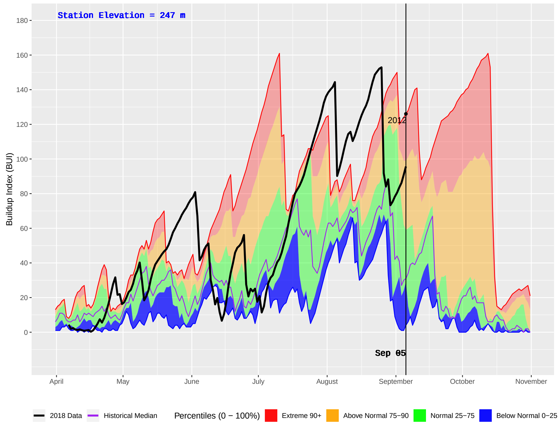
FORD MOUNTAIN (1144) : Historical (2012–2016) and Current (2018) Daily Buildup Index (BUI)
