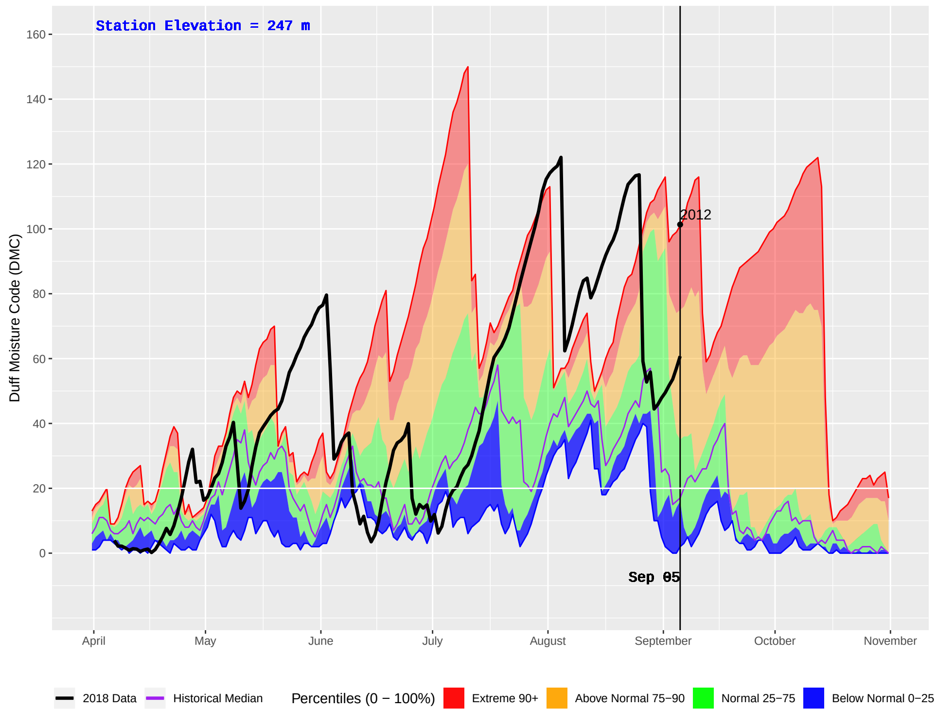
FORD MOUNTAIN (1144) : Historical (2012–2016) and Current (2018) Daily Duff Moisture Code (DMC)
