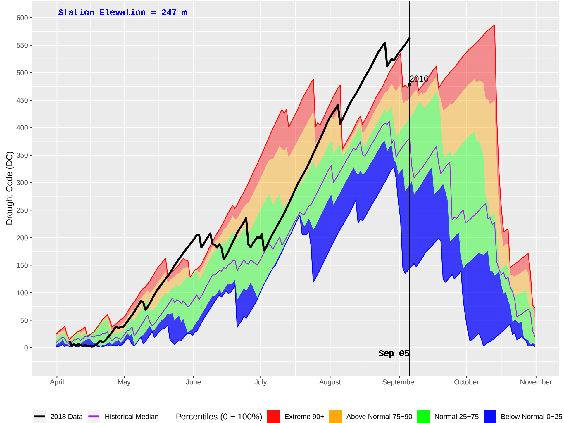
FORD MOUNTAIN (1144) : Historical (2012–2016) and Current (2018) Daily Drought Code (DC)
