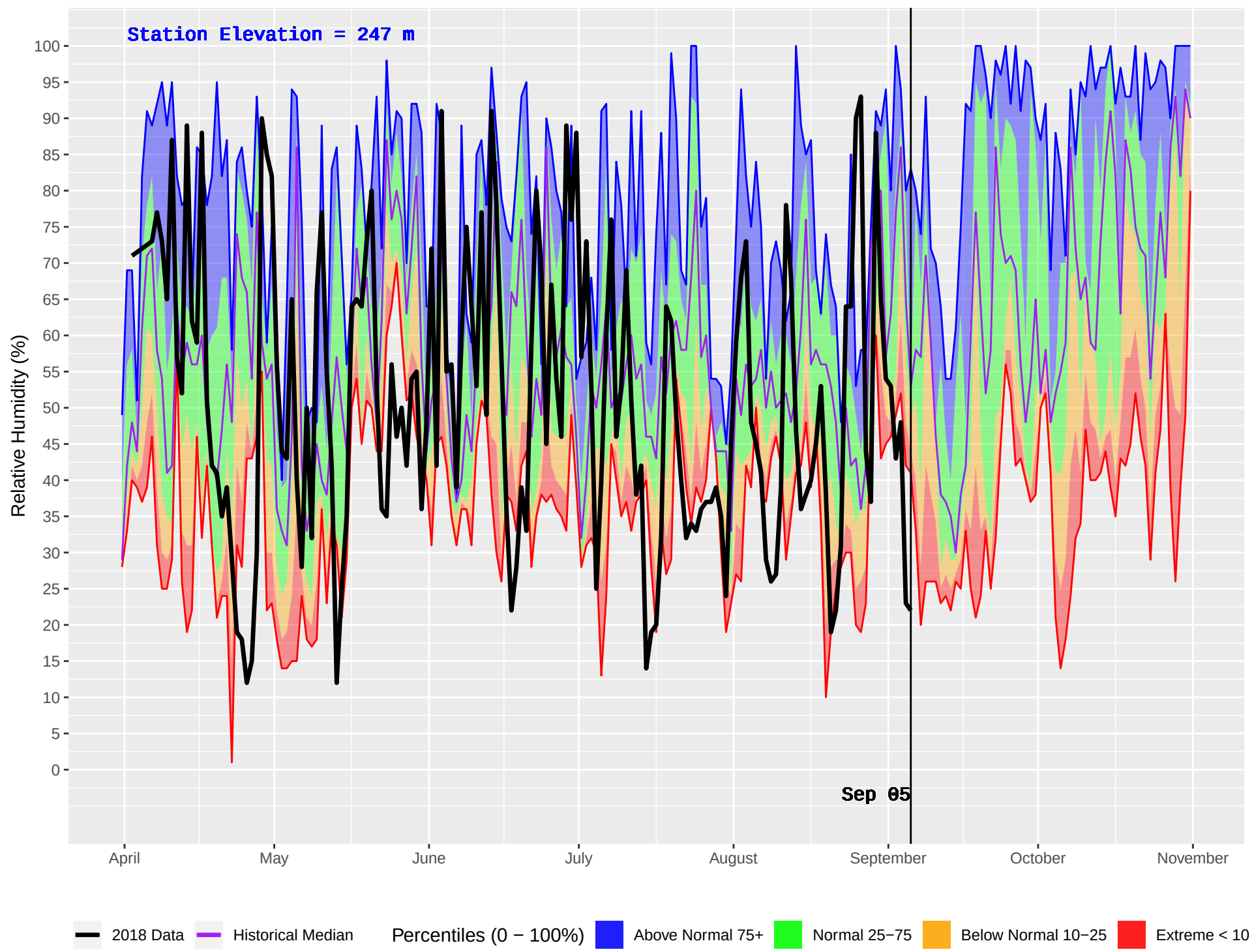
FORD MOUNTAIN (1144) : Historical (2012–2016) and Current (2018) Daily Relative Humidity
