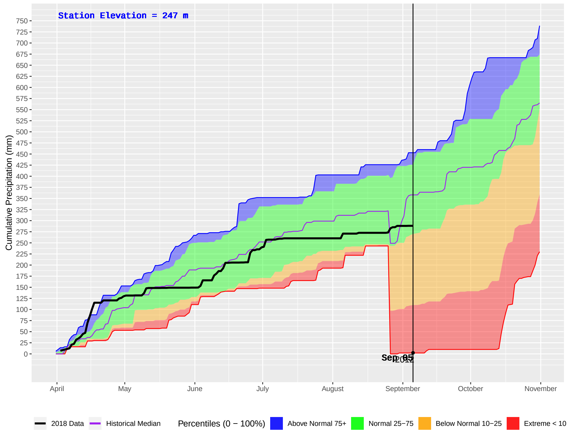
FORD MOUNTAIN (1144) : Historical (2012–2016) and Current (2018) Daily Cumulative Precipitation
